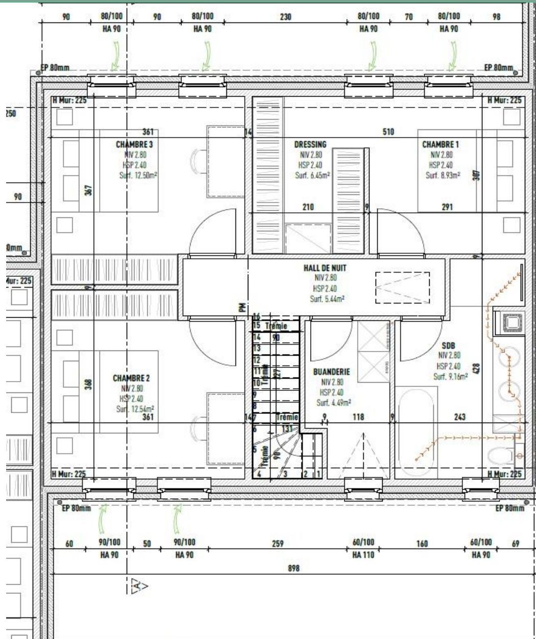
Plan Rez+1 - Lots 9-10-11 Echelle 1/50
